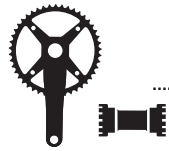
FC-MX71 HOLLOWTECH II crank w/BB unit w/o gear SM-CR80-A single gear 34/38/41/42/43/44/46T
